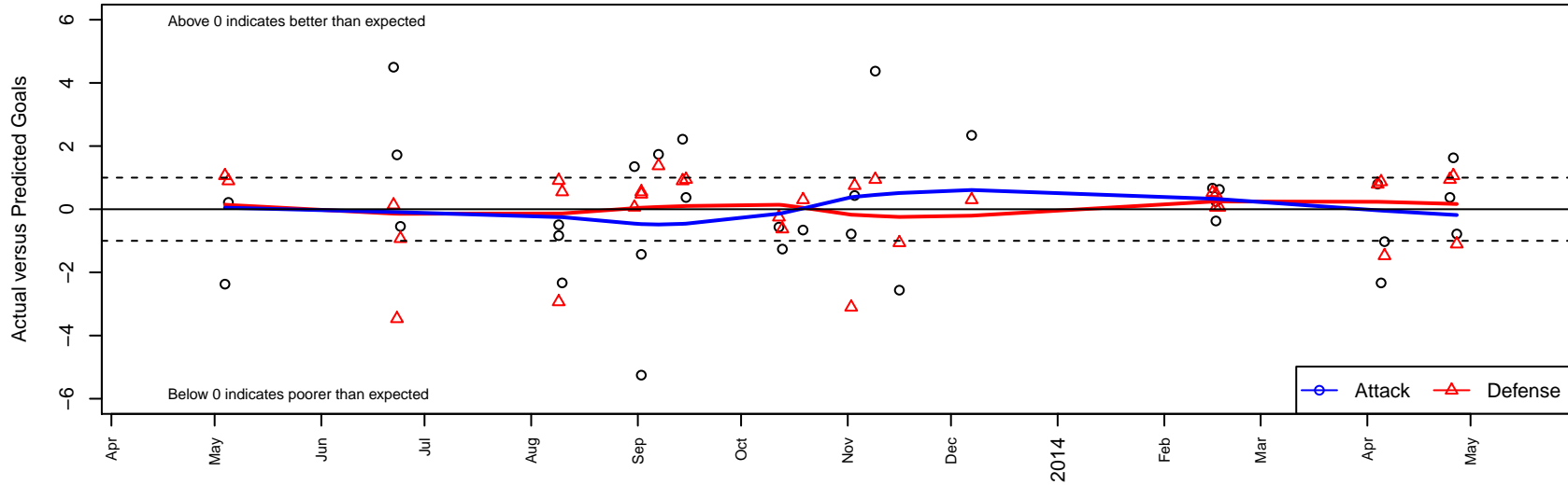
MV Bombers B99 Dots are actual minus expected GF (blue circles) and GA (red triangles). Blue line is smoothed change in attack strength. Red is smoothed change in defense strength.
